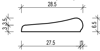
MEDITERAN 27,5cm; l=60cm
