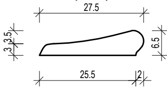
DUNAV 25,5cm; l=60cm
